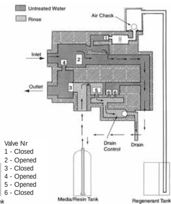
C7 Fast Rinse 2 position
