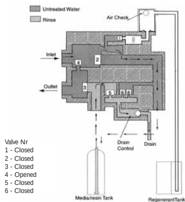
C4 System Pause position (repressurize)
