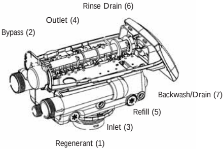
C0 Treated water position (normal position)
