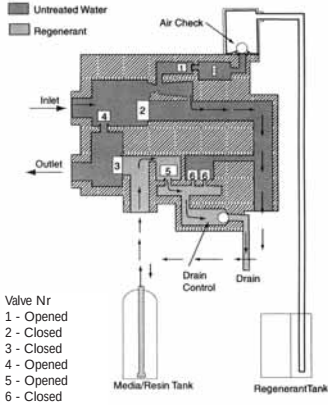
C3 Slow Rinse position
